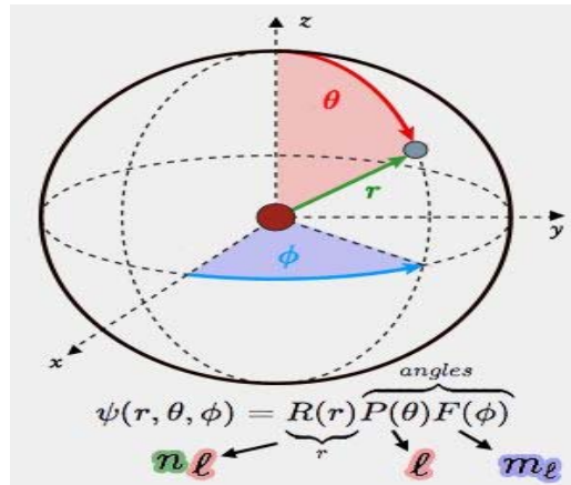
Spherical coordinates
