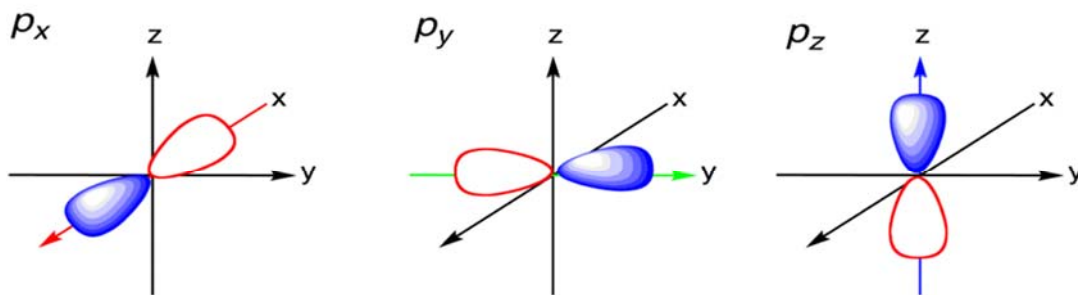
The three p orbitals are aligned along perpendicular axes
