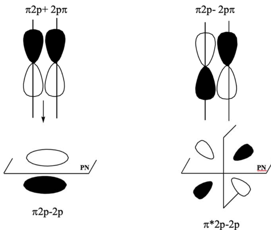
Representation of the lateral overlap of two O.A.p
