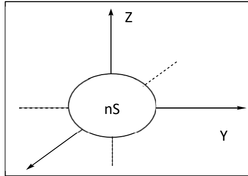
The orbital (ns)
