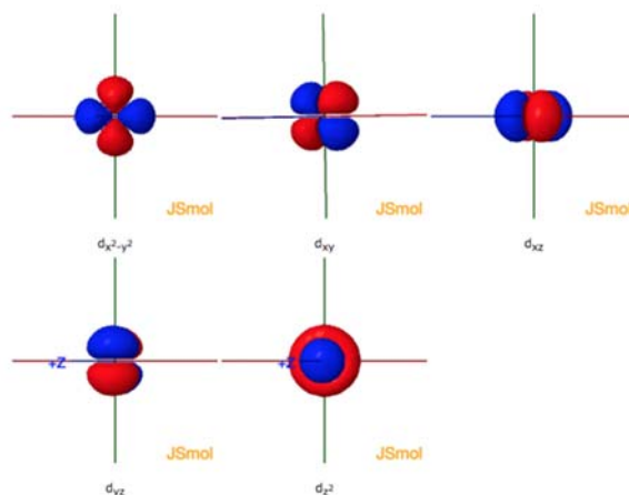
The orbital (nd)
