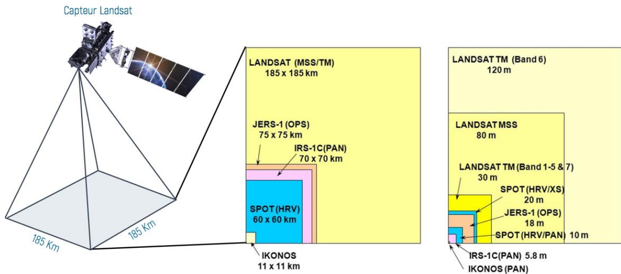
Figure N° 10: The swath of some satellites with their spatial resolutions. Source : Mohand Bersi 2018
