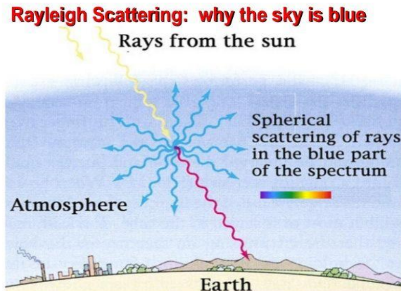
Figure N° 09: Rayleigh scattering
