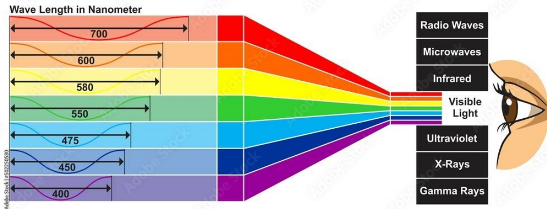
Figure N° 03: The different types of EMR and their wavelengths.
