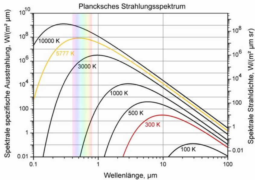
Figure N° 10: Planck radiation spectra for different temperatures, in log-log representation Source : https://www.techno-science.net/glossaire-definition/Loi-de-Planck-page-3.html
