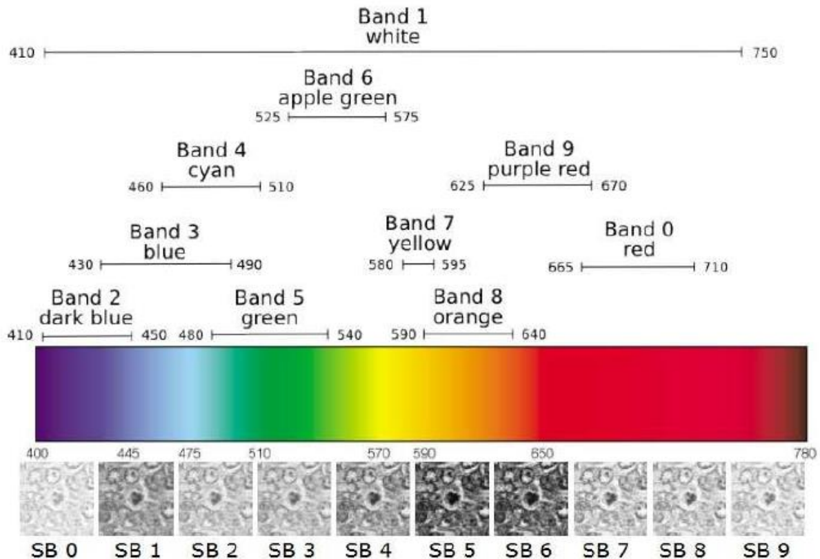
Figure N° 12: Spectral bands of the multispectral microscope. Source : Source : Mohand Bersi 2018
